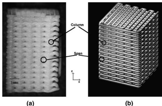
Fig. 2. (a) Side view of the tower architecture and (b) an idealized 3-D schematic.
