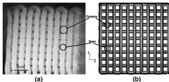
Fig. 1. (a) Top view of an alumina tower and (b) an idealized schematic illustrating the layering pattern.
