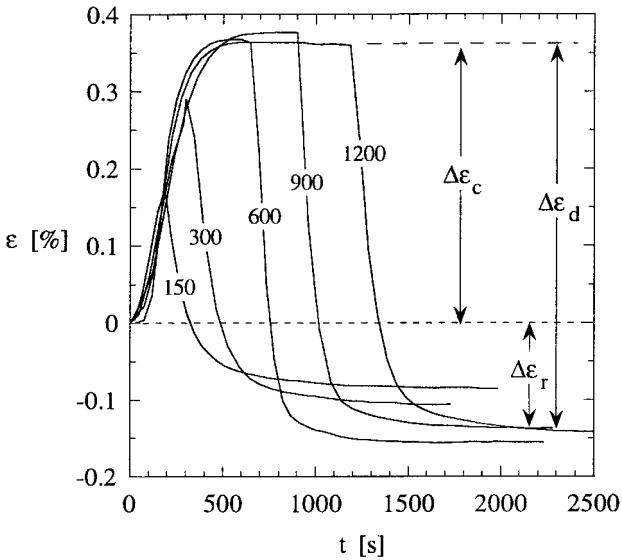
Figure 2. Strain history of titanium specimens during dilatometric hydrogen cycling experiments at 860^{\circ}\text{C} . Each curve is labelled with the charging time, t_c , in seconds, and the strain of charging ( \Delta\varepsilon_c ), strain of discharging ( \Delta\varepsilon_d ), and chemical ratchetting strain ( \Delta\varepsilon_r ) are shown schematically for the longest experiment ( t_c = 1200\text{ s} ).
