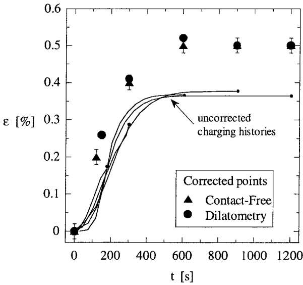
Figure 6. Strain history during hydrogen charging at 860^{\circ}\text{C} , including uncorrected, experimental data from figure 2, and data points corrected to remove ratchetting shrinkage. Ratchetting data from both contact-free and dilatometric experiments have been used in the correction.
