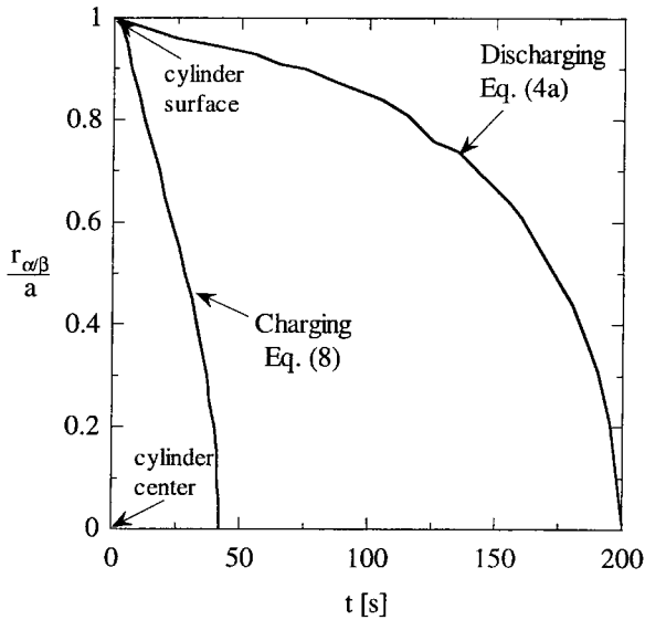
Figure 8. Radial position of the \alpha - \beta phase transformation front during both charging and discharging at 860^\circ\text{C} , as given by equations (8) and (4a), respectively.
