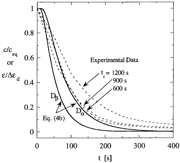
Figure 4. Strain history during hydrogen discharging at 860^{\circ}\text{C} for charging times t_c , normalized by the total discharging strain, \Delta\varepsilon_d . Shown for comparison are concentration histories, c/c_{eq} , predicted by equation (4b), using D_\alpha or D_\beta for the diffusivity of hydrogen in titanium, D .
