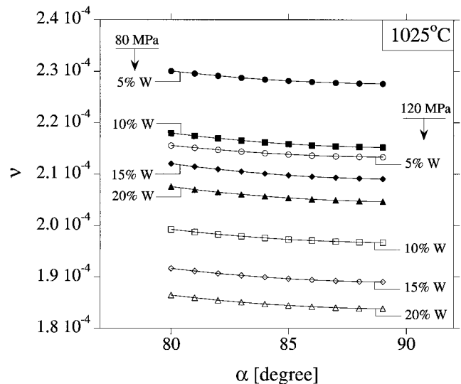
Fig. A2—Variation of \nu with choice of \alpha between 80 and 89 deg for the determination of the third boundary condition, for different tungsten fiber volume fractions at composite stresses of 80 and 120 MPa for NiAl-W composites at 1025 °C.
